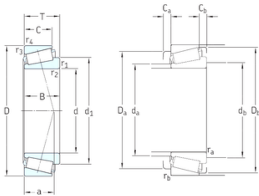
Bearing No. 30302J2
